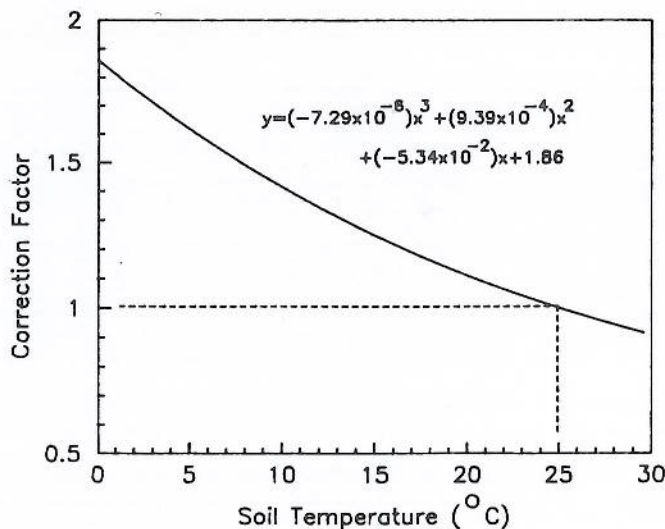
Fig. 1. Temperature correction curve for EC a readings (derived from Richards (1954)).
