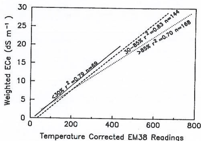
Fig. 4. Linear regressions of temperature-corrected EM38 horizontal mode readings with weighted \text{EC}_e for three moisture classes on a medium-textured soil.
