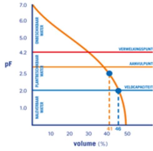
Figuur 18. pF curve bodemonmonster
